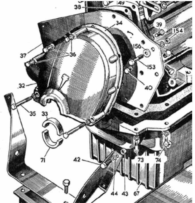
Illustration of the MG TF Engine from the Factory Parts Book.
